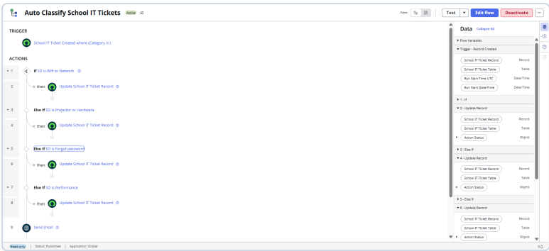
Figure 1: Published Auto Classify School IT Tickets Flow Designer workflow used for functional test execution.
